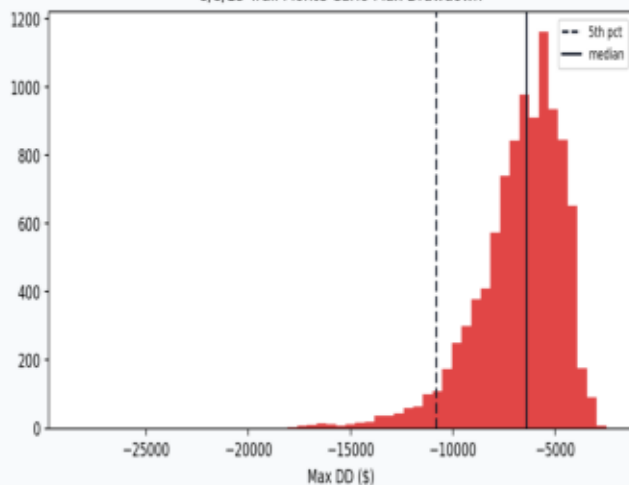
8/8/15 Trail Monte Carlo Max Drawdown
