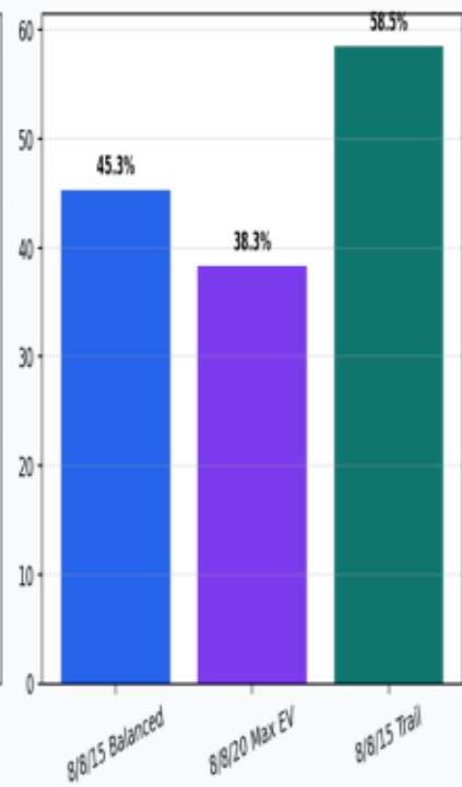
Win Rate
