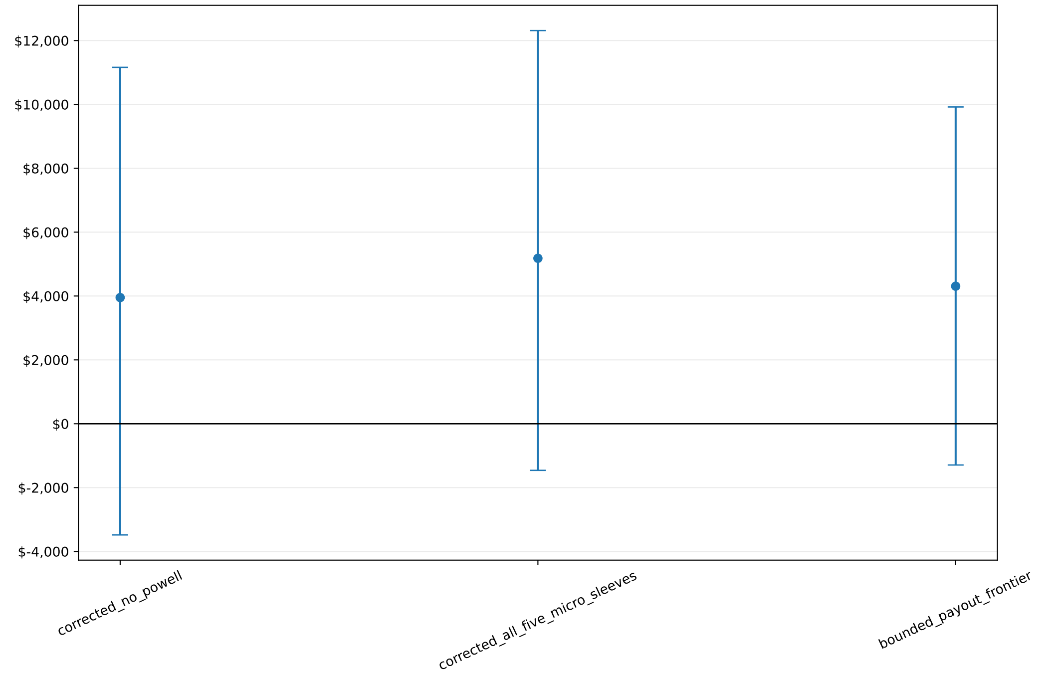
21-session Monte Carlo: mean with P05/P95
